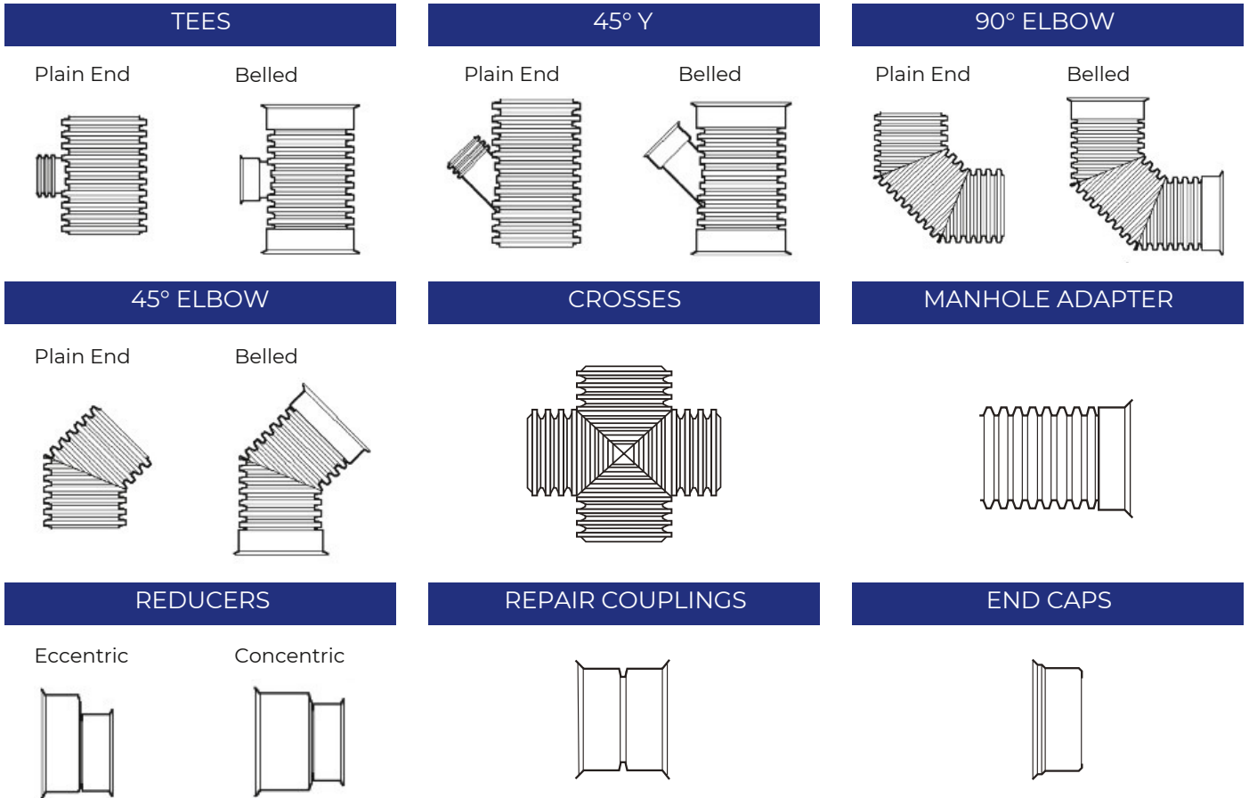
FIGURE 4: Fitting Configurations
